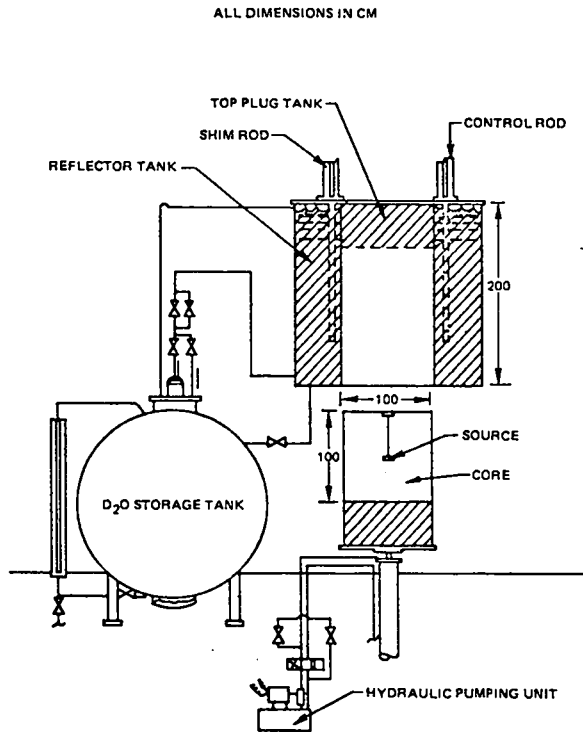
Fig. A-1. Los Alamos Scientific Laboratory cavity reactor assembly.
